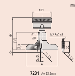
7231 A= 63.5mm
